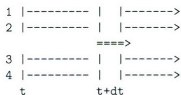
Sketch 1. Parallel solution of the set of N Kohn–Sham equation ( N = 4 ). The double line == indicates the serial phase in which each slave processor forwards its partial density to the master and subsequently receives the effective potential to initiate the next step.
