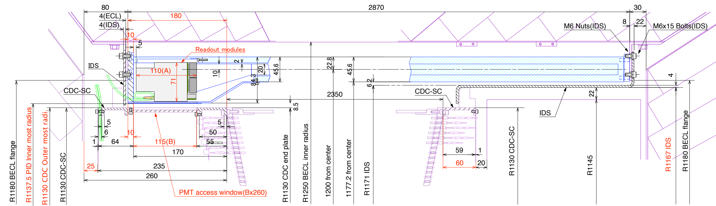
Backward IDS and QBB detail : Scale 1/2
