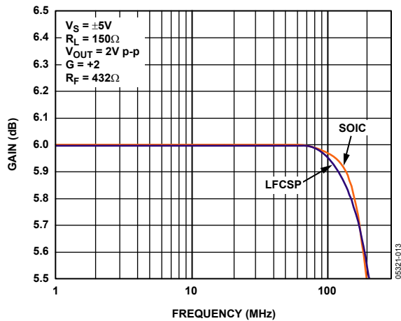
Figure 13. 0.1 dB Flatness
