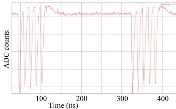
Figure 6: digitized waveform from current readout system. The display shows 5 bunches with 14ns separation in trains with 280ns separation.
