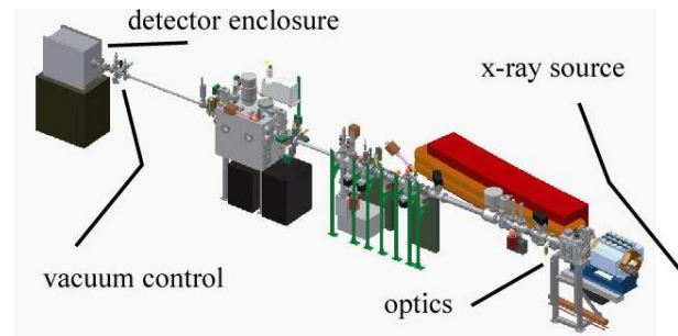
Figure 1: layout of the xBSM (positron line)
