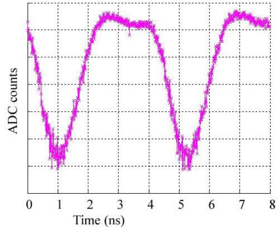
Figure 7: digitized waveform from fast preamplifiers and 4ns digitizer
