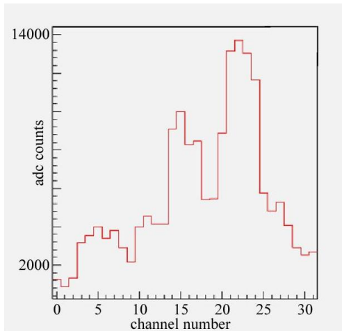
Figure 5: Coded Aperture
