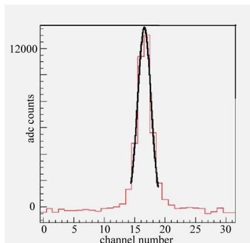
Figure 3: vertically limiting slit with Gaussian fit
