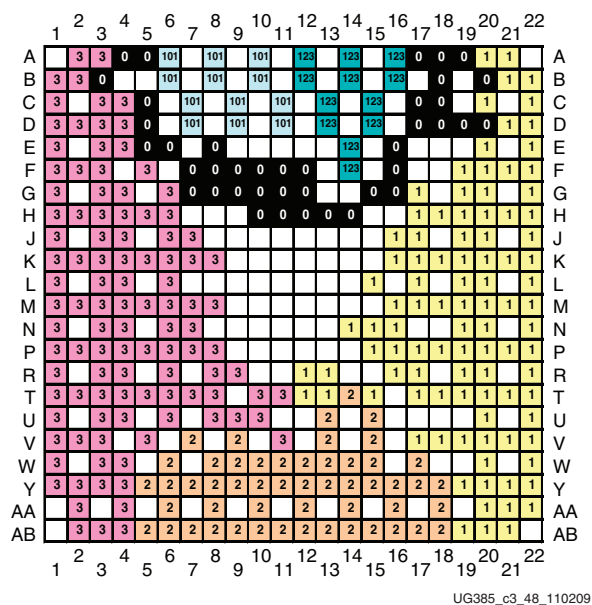
Figure 3-48: CS(G)484 Package—LX45T, LX100T, and LX150T I/O Bank Diagram
