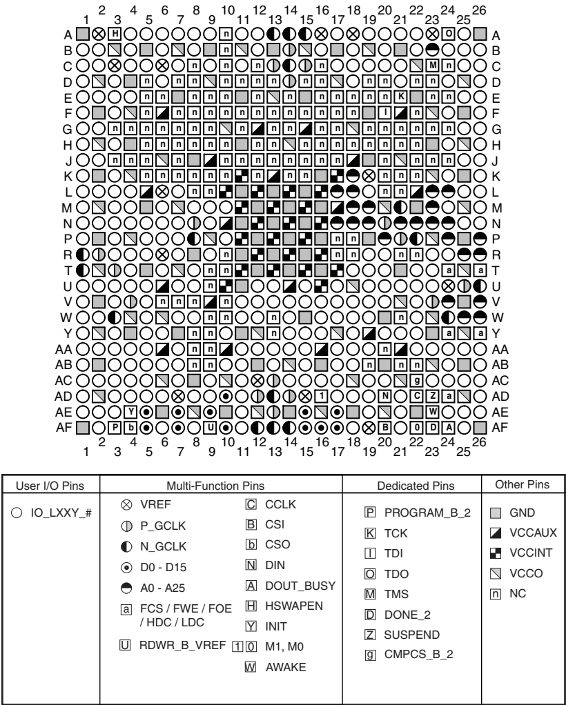
Figure 3-49: FG(G)676 Package—LX45 Pinout Diagram
