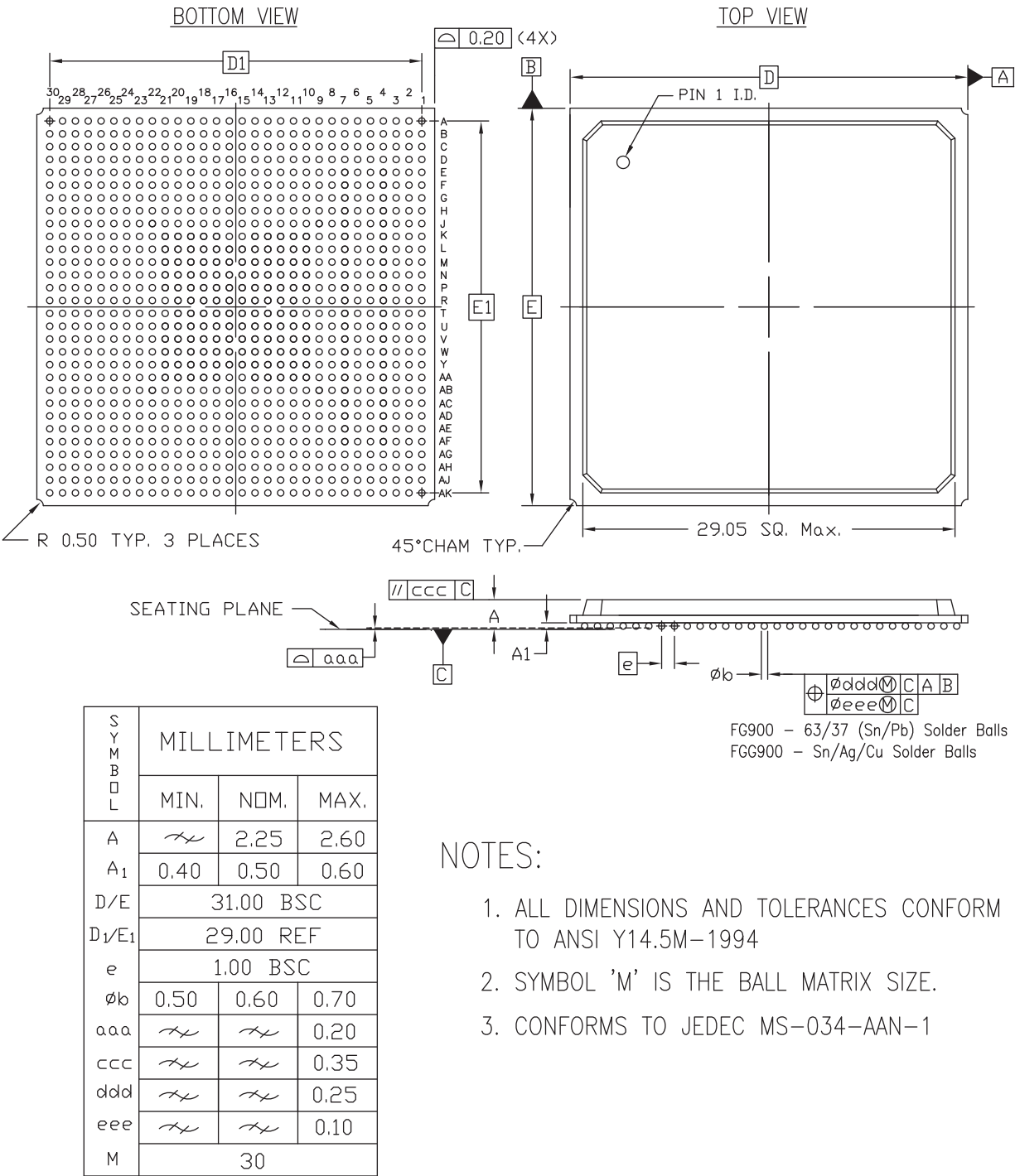
Figure 4-8: FG(G)900 Chip-Scale BGA Package
