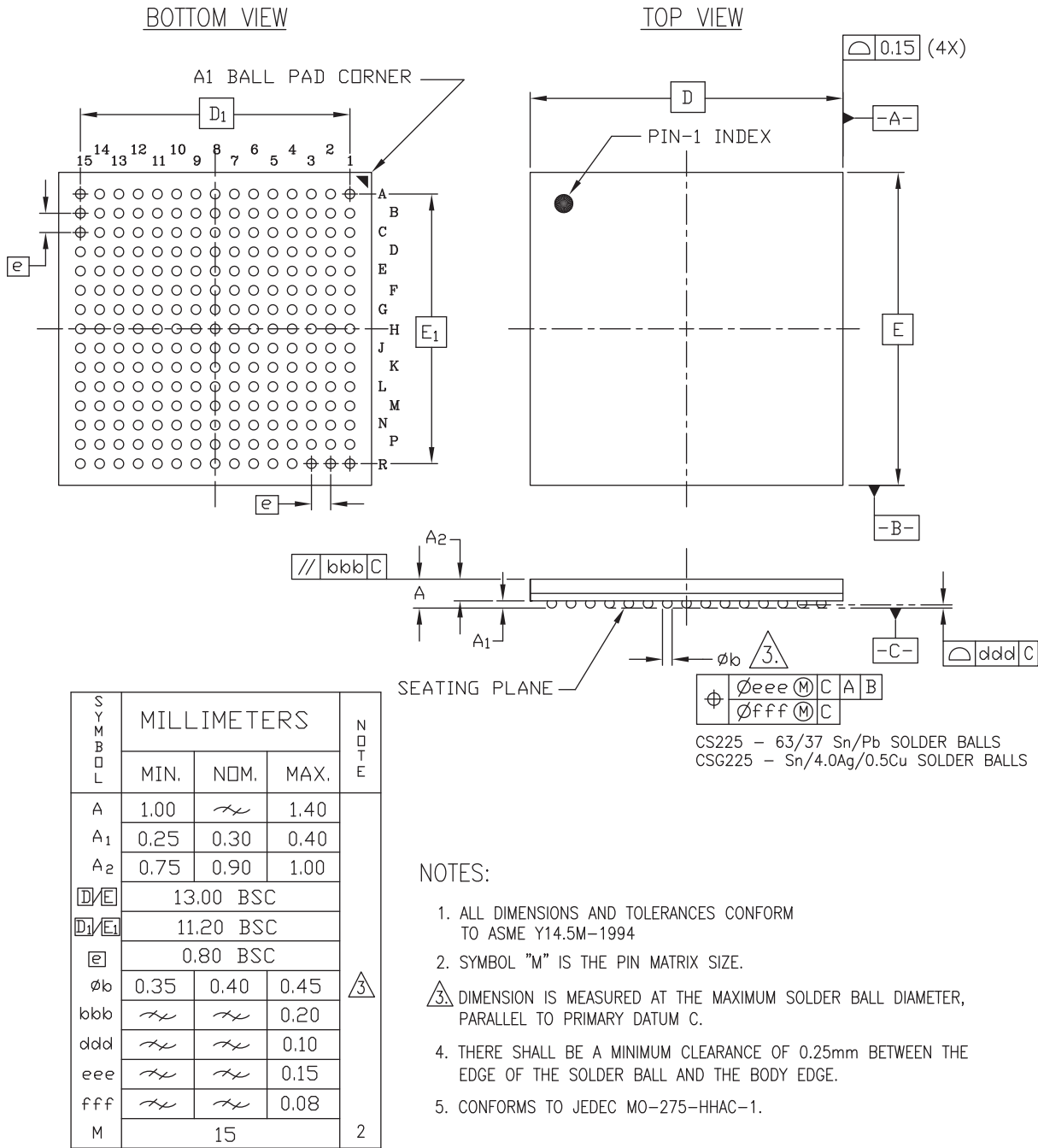
Figure 4-3: CSG225 Chip-Scale BGA Package
