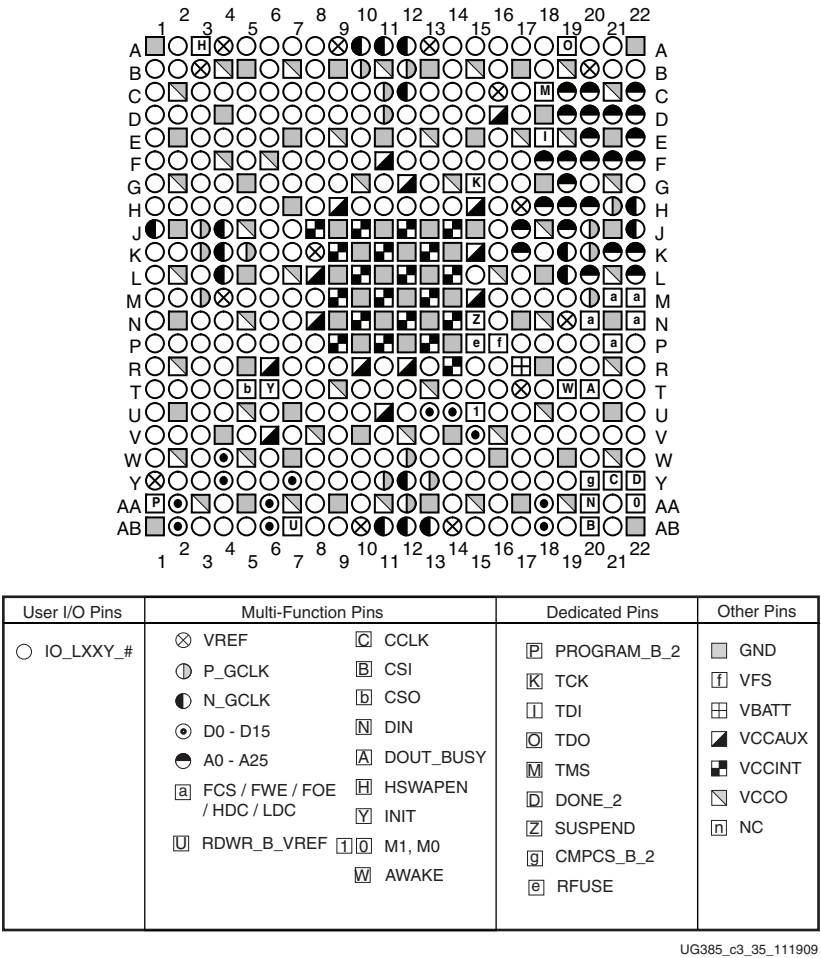
Figure 3-35: FG(G)484 Package—LX150 Pinout Diagram
