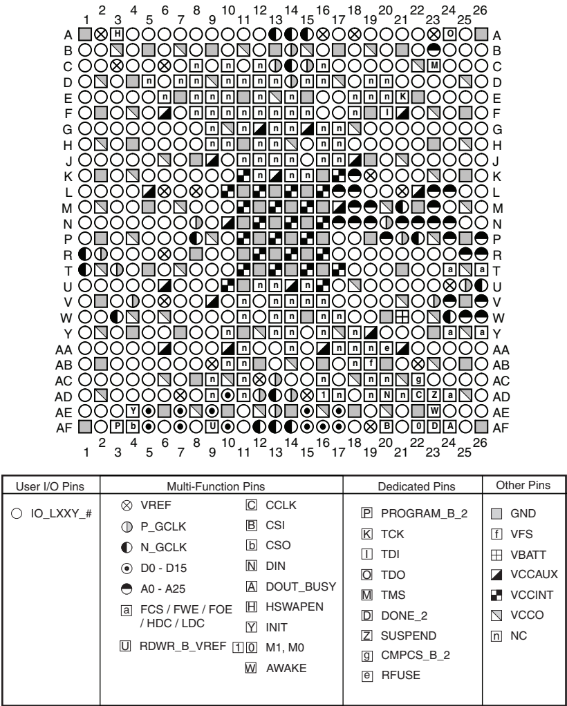
Figure 3-51: FG(G)676 Package—LX75 Pinout Diagram
