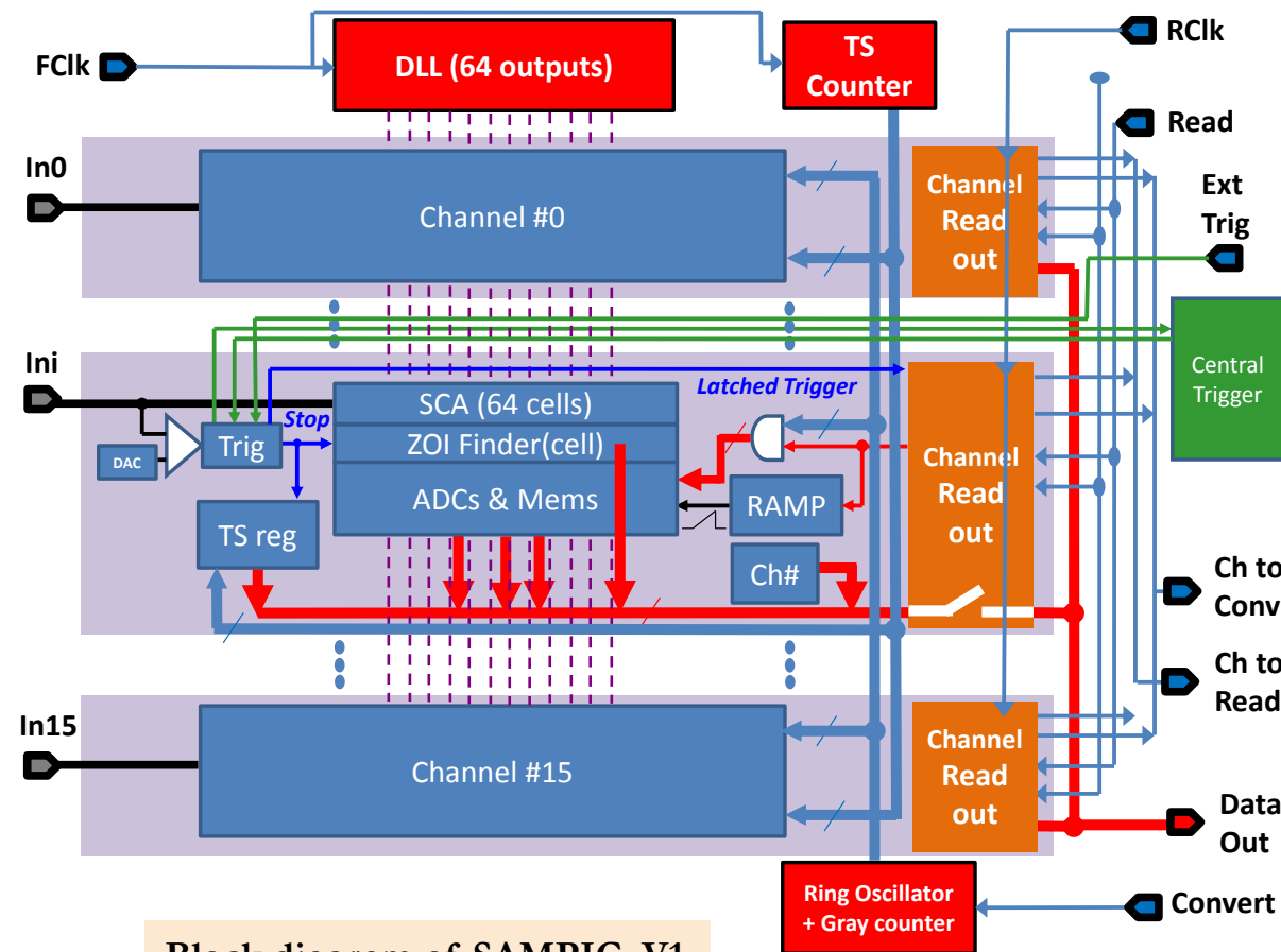
Block diagram of SAMPIC_V1
