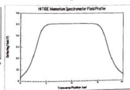
Figure 7. (Bottom left) Simulated magnetic field profile for the magnet shown in Figure 6a.
