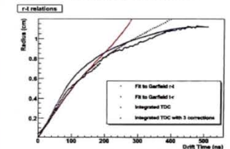
Figure 5. Relationships between the radius of closest approach of the muon track to the drift tube wire and the time of first signal on the drift tube. The brown and red points indicate fits to the simulated results. Light blue indicates a first estimate based on the timing signals seen in the drift tubes. This is further refined using an iterative correction procedure. The points in dark blue indicate the results after 3 iterations.
