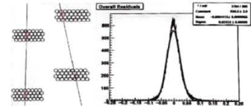
Figure 8. (Left) Projections of a reconstructed muon path through the two pairs of superlayers. Red circles indicate a tube with a measured hit. Blue circles represent the expected distance of closest approach in tubes through which the track passes. (Right) Measurement of muon impact parameter residuals after optimization of the drift time relation. The line is fit to a Gaussian with a width of approximately 2.5 microns.
