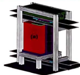
Figure 6. (Top left) CAD rendering of the momentum spectrometer assembly. The red box is the 0.5 T magnet. Above and below the magnet are pairs of DSSDs. The green box above the upper DSSDs is an area for testing prototype vertexing devices.
