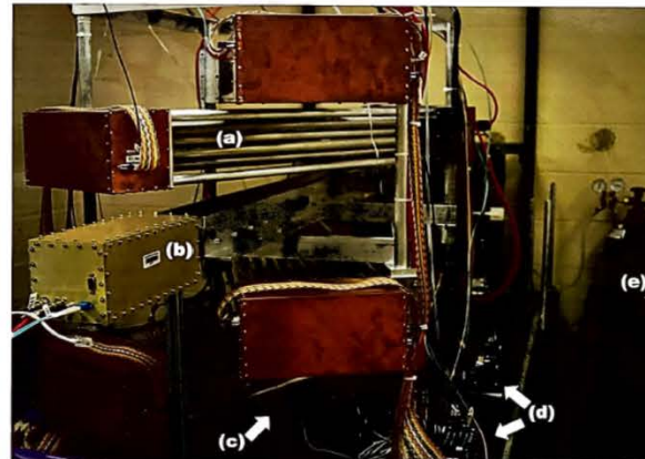
Figure 2. Photograph of the current muon beamline systems. Most components are mounted to the optical bench for ease of alignment.
