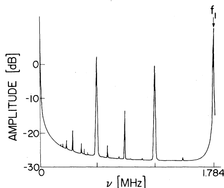
FIG. 7. Period tripling.
