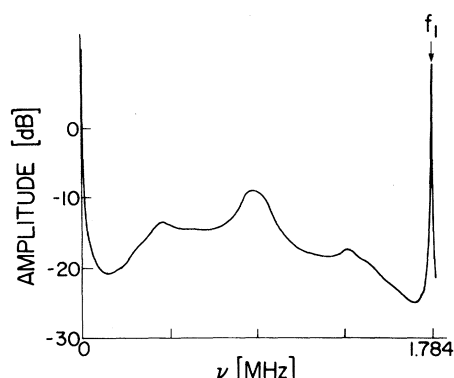
FIG. 4. Fully developed chaotic spectrum.
