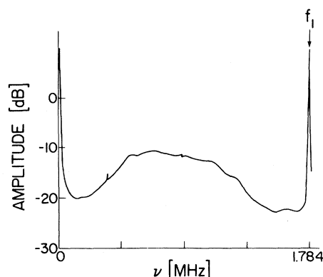
FIG. 6. Secondary chaotic spectrum.
