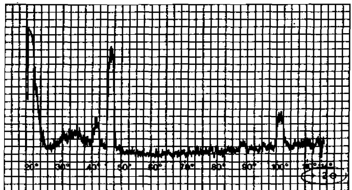
Fig. 15.7 LiF 20 kV
