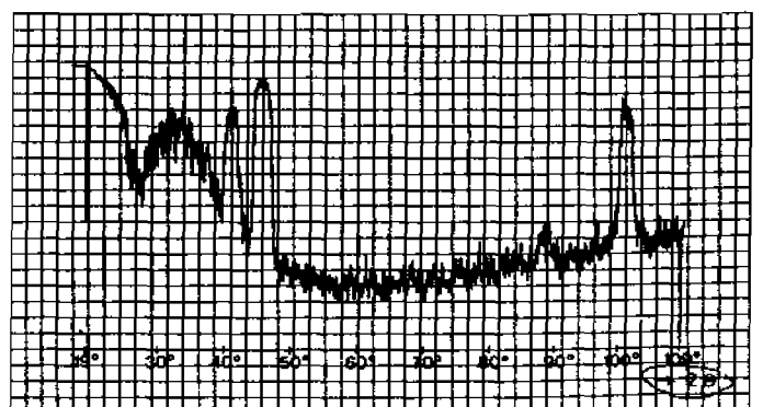
Fig. 15.8 LiF 30 kV
